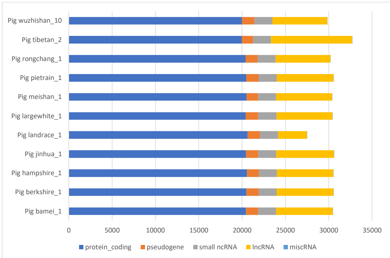
Figure 2: Counts of the major gene classes in each species
