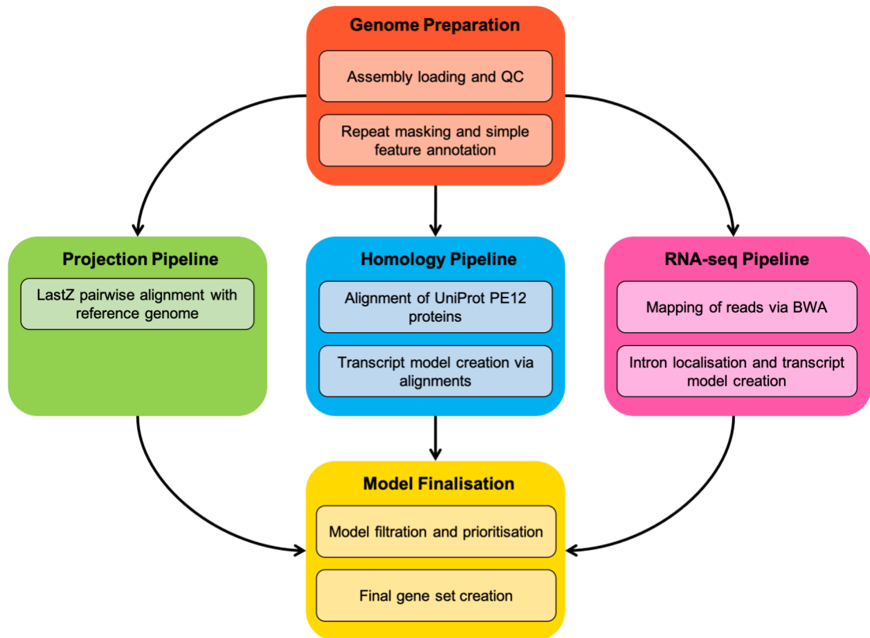
Figure 1: Flowchart of the protein-coding annotation pipeline. Small ncRNAs, Ig genes, TR genes, and pseudogenes are computed using separate pipelines. For pigs annotation, we also used Iso-seq pipeline.
