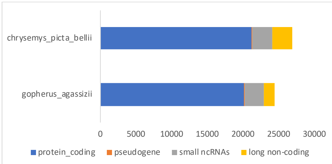
Figure 2: Counts of the major gene classes in each species
