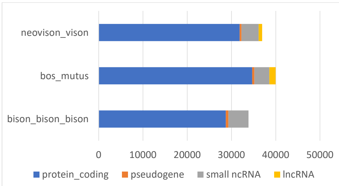
Figure 3: Counts of the major transcript classes in each species
