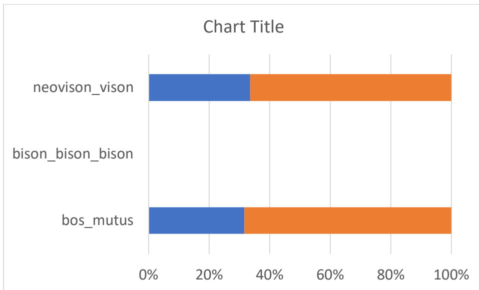
Figure 5: Number of bases unmasked (orange) and repeat masked (blue) per species using the custom RepeatModeler repeat libraries (where available)
