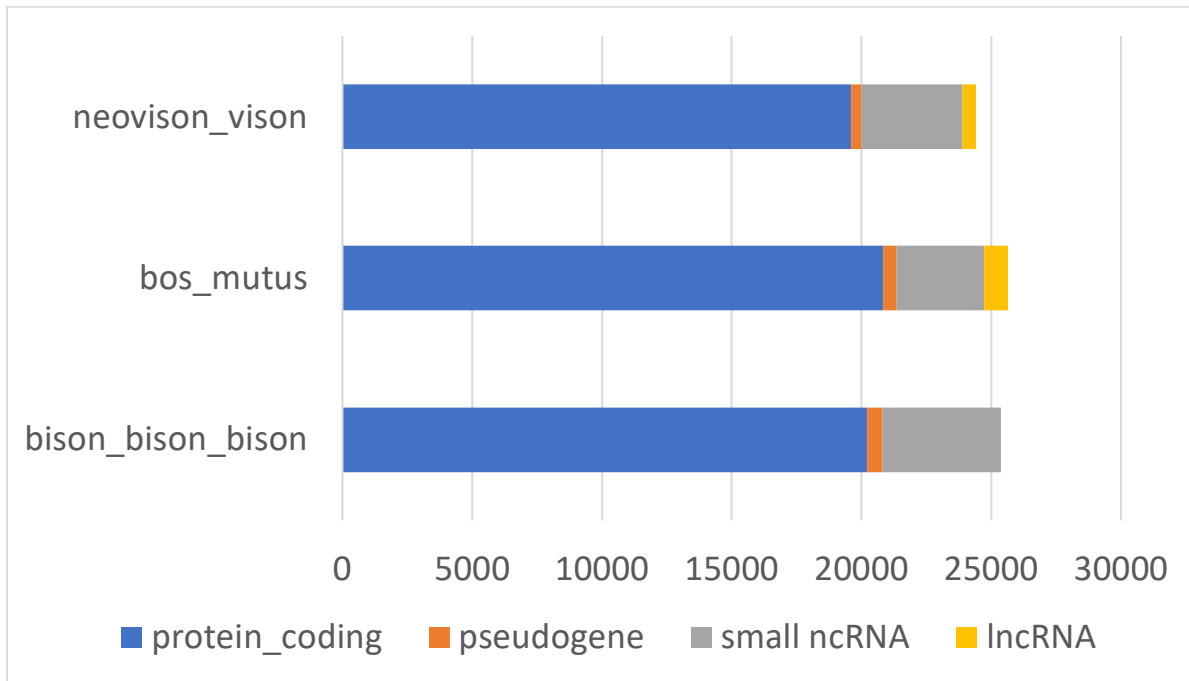
Figure 2: Counts of the major gene classes in each species
