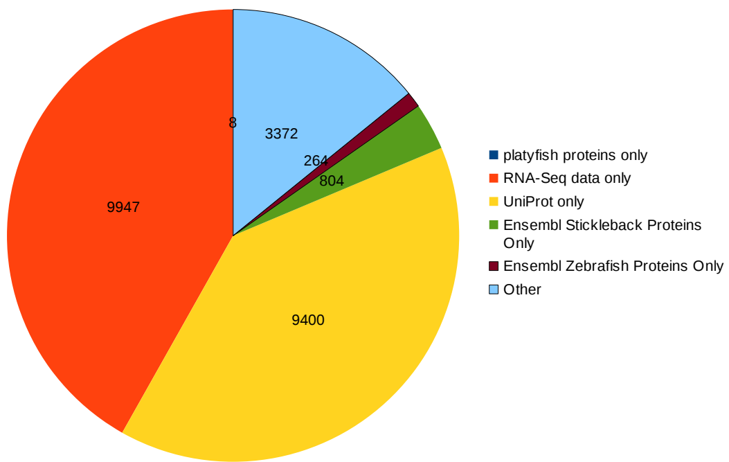
Figure 4: Supporting evidence for platyfish final gene set
