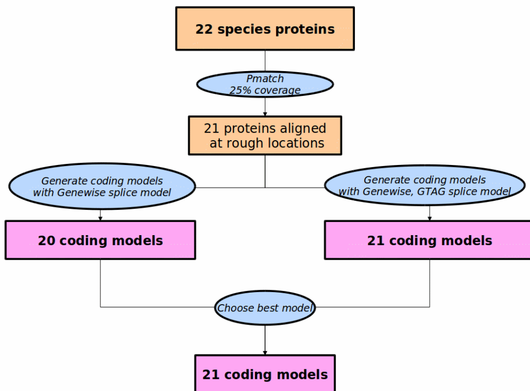
Figure 2: Targeted stage using platyfish protein sequences.
