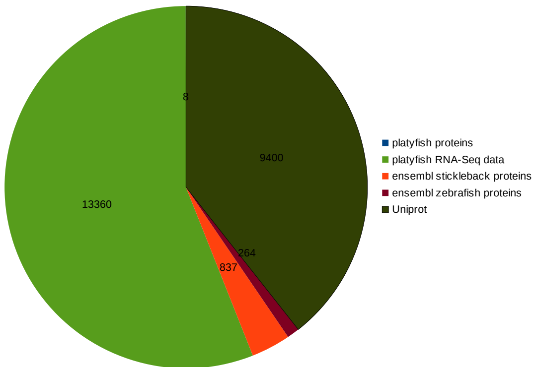
Figure 5: Supporting evidence for platyfish final transcript set
