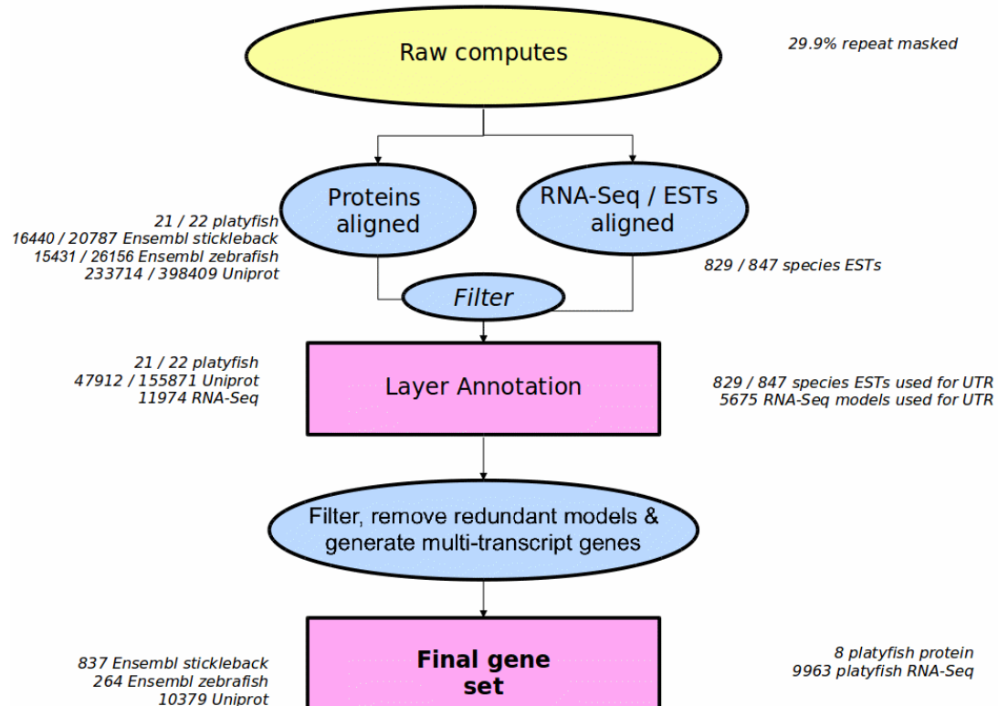
Figure 1: Summary of platyfish gene annotation project
